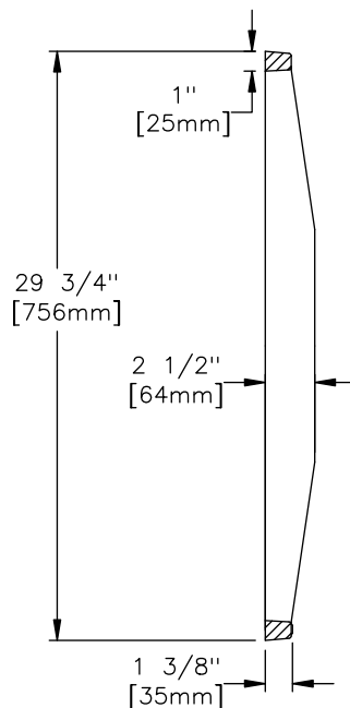
SECTION
